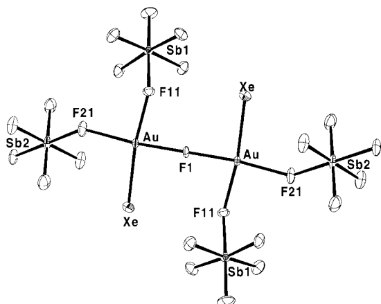
Figure 4. Structure of the [\text{Xe}-\text{Au}-\text{F}-\text{Au}-\text{Xe}]^{3+} ion and its closer anion environment in [\text{Au}_2\text{Xe}_2\text{F}^+][(\text{SbF}_6)^-]_3 ( 4 ; (ORTEP representation with 50% probability ellipsoids); selected bond lengths [pm]: Au–Xe 264.7(1), Au–F1 204.5(2), Au–F11 216.6(4), Au–F21 218.9(4), Sb1–F11 194.0(4), Sb2–F21 193.7(4).
